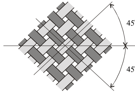
Plain Woven Fabric: Free State
