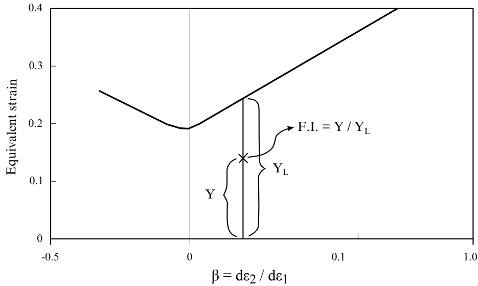
Figure M37-2. Calculation of F.I. based on critical effective strain method.
